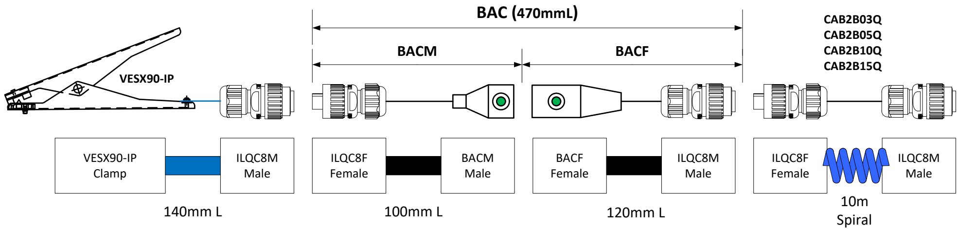
BAC GA Drawing 1V0 27/05/2021
